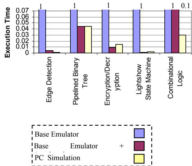
Figure 10: Performance of SystemC emulator (normalized to the base emulator). In some examples, the emulator with acceleration was able to perform faster than the same SystemC circuit running on a PC.
