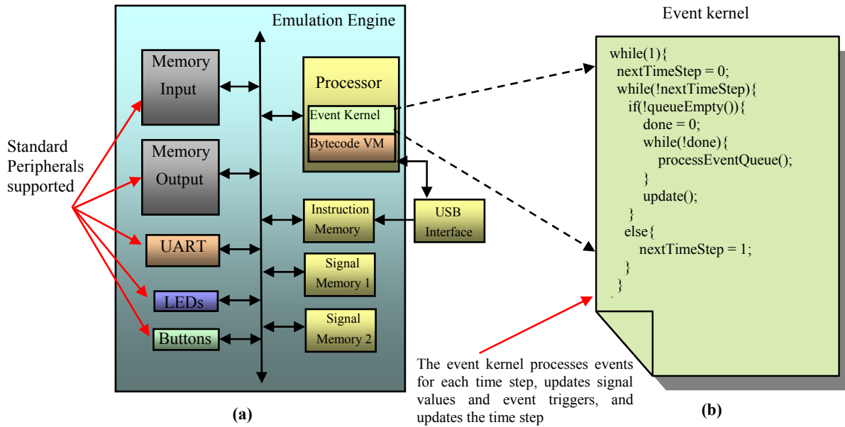
Figure 5: Basic emulation engine. The emulation engine consists of a hybrid event-driven kernel to allow a variety of different circuit implementations. Circuits can also take advantage of a range of standard peripherals, including lights, buttons, a UART, and input and output memories.
