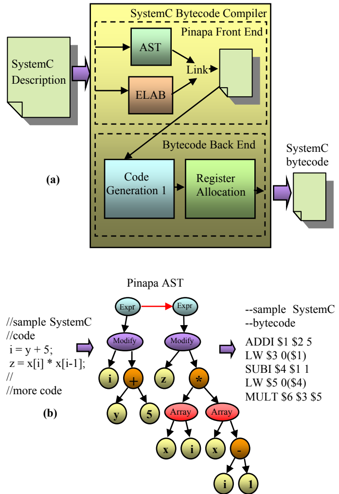
Figure 2: SystemC bytecode compiler: (a) The SystemC bytecode compiler builds on PINAPA , a SystemC front-end tool, and uses a custom SystemC bytecode backend; (b) Sample code generation during the first phase of the SystemC bytecode back end.
