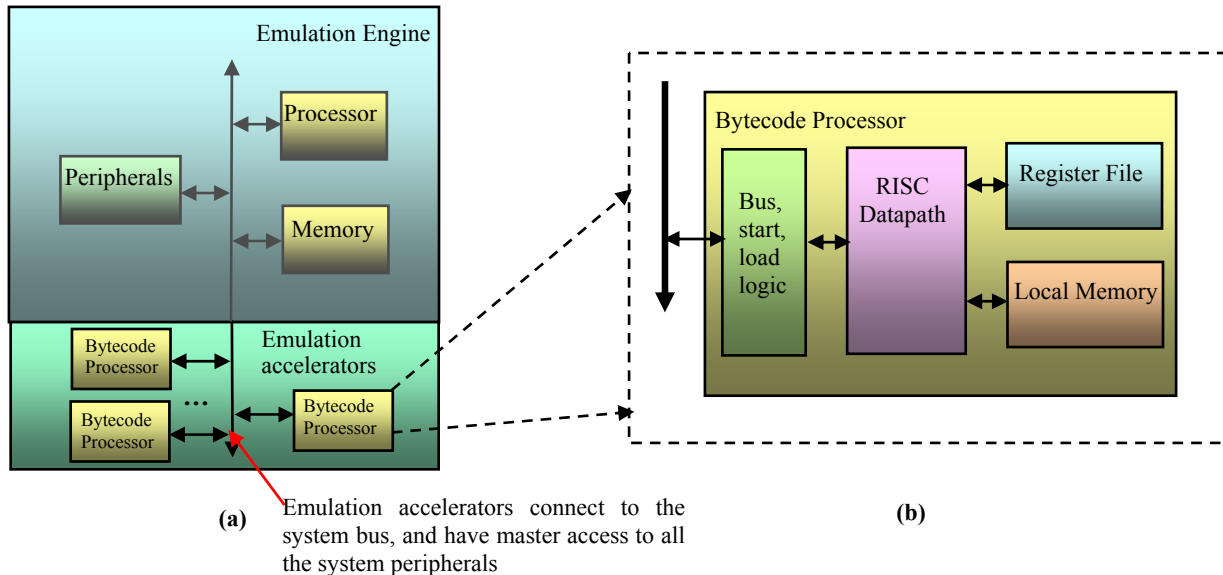
Figure 6: Emulation accelerators. The emulation accelerator consists of a multicycle MIPS-like datapath than can execute one instruction in about 3-4 cycles, almost 100X faster than executing the same instructions in the base emulator.
