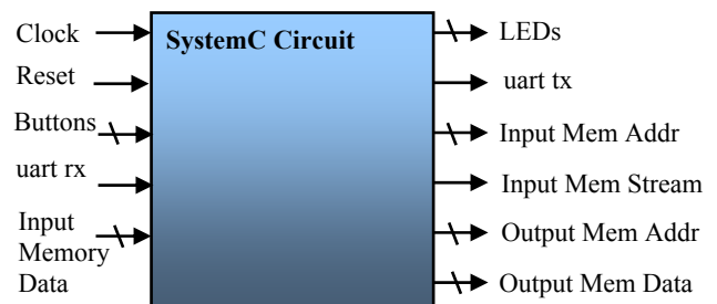
Figure 7: SystemC-on-a-Chip circuit interface. The emulation engine supports access to multiple peripherals, including buttons, LEDs, and memory.
